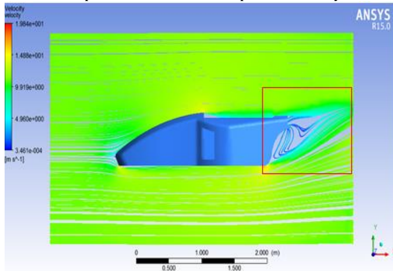
Figure 4. The streamlined flow pattern on the car body
