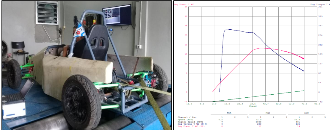
Figure 6. Dynotest
